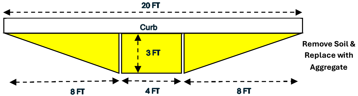
Horizontal/Side View
